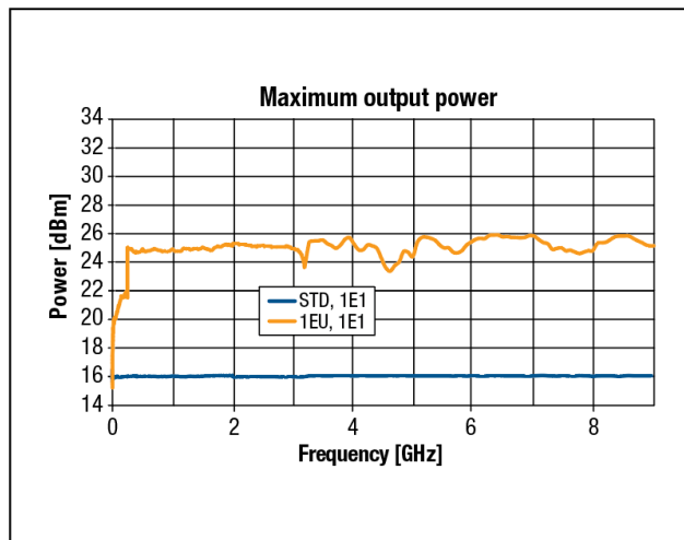
Maximum output power (measured)
