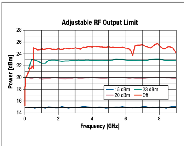
RF output limit (measured)
